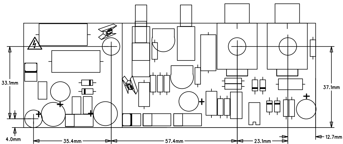
PCB Top Components View
